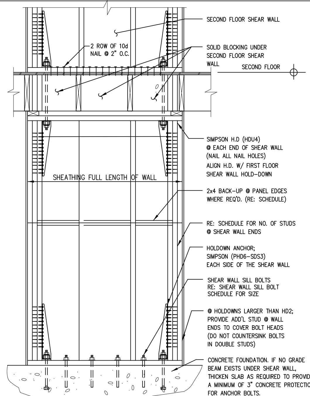
TYPICAL SHEAR WALL DETAILS (W/ UPPER FLOOR HOLD- DOWN)
