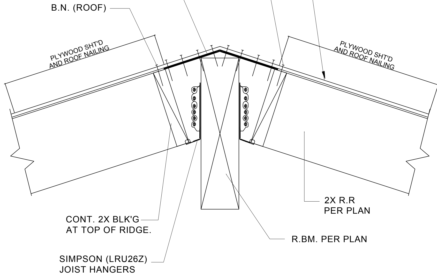
1 RAFTER TO RIDGE CONNECTION SCALE:N.T.S
