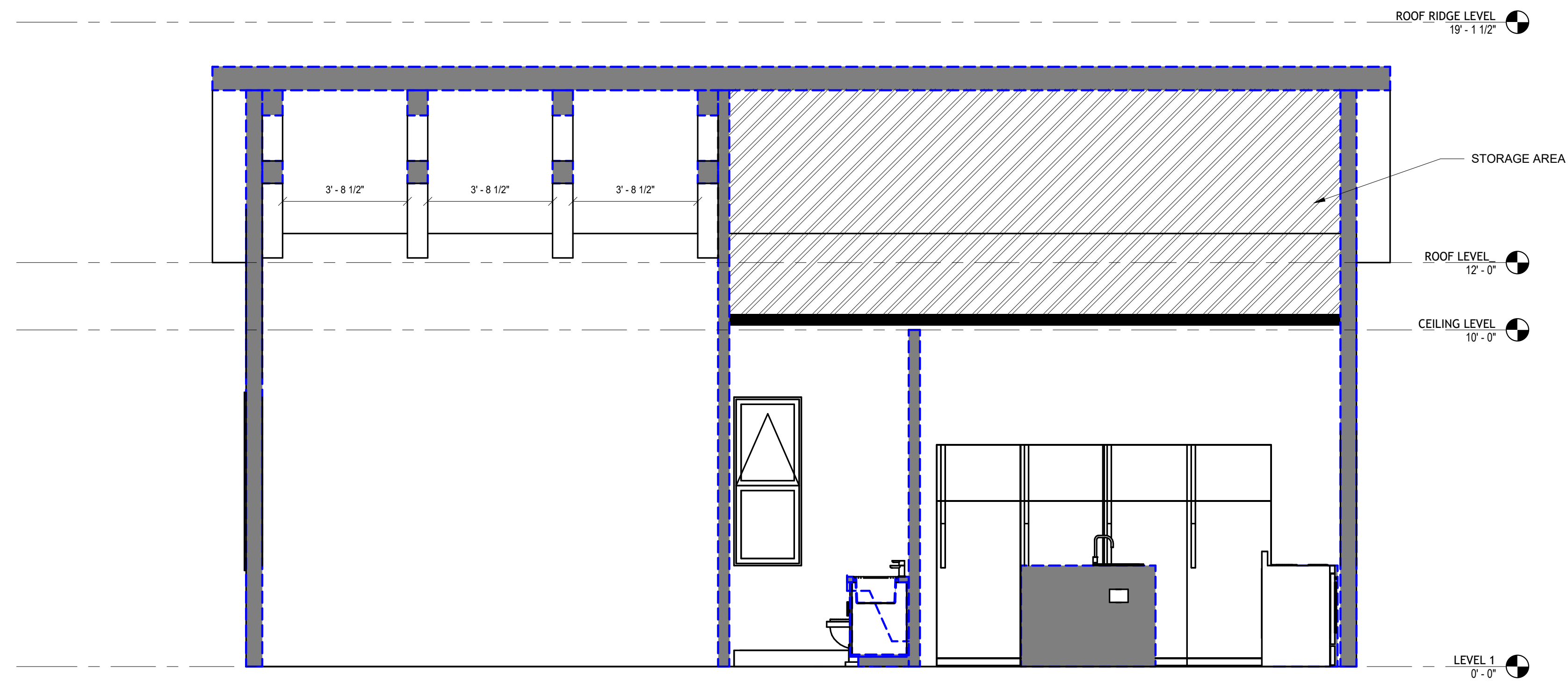
3 | Section 3 3/8" = 1'-0"
