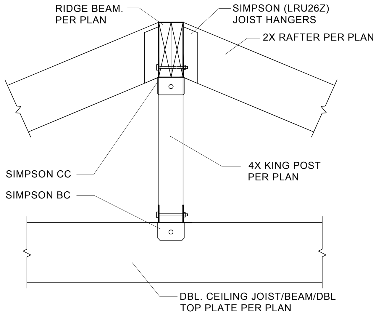
2 KING POST TO BEAM CONNECTION SCALE:N.T.S
