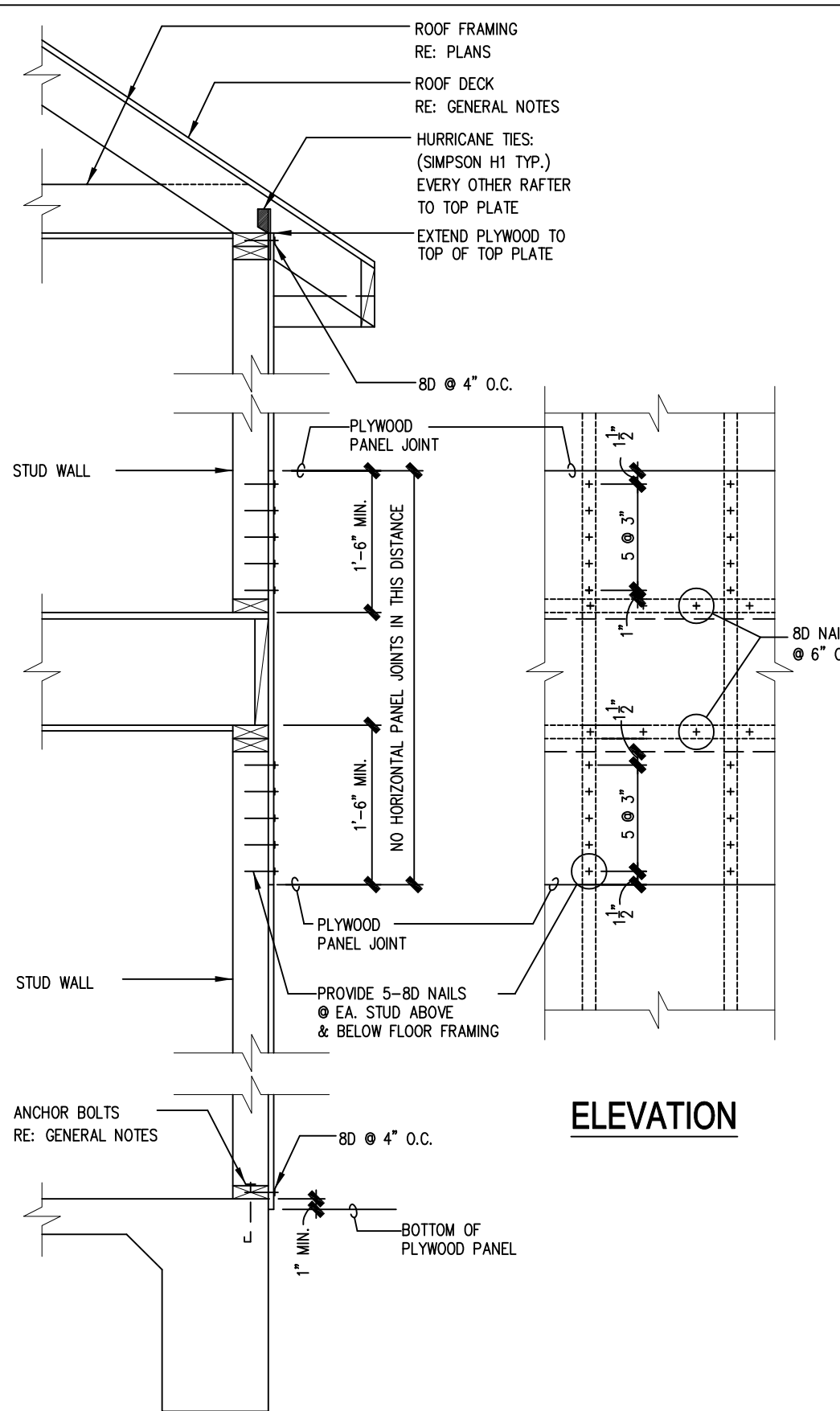
TYPICAL WIND STRAPPING DETAILS (PLYWOOD OPTION)
