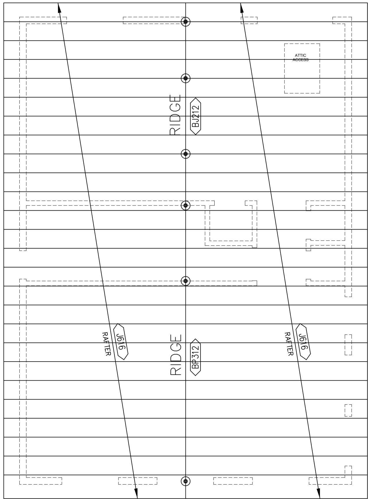
ROOF PLAN SCALE: 1/4"= 1'-0"
