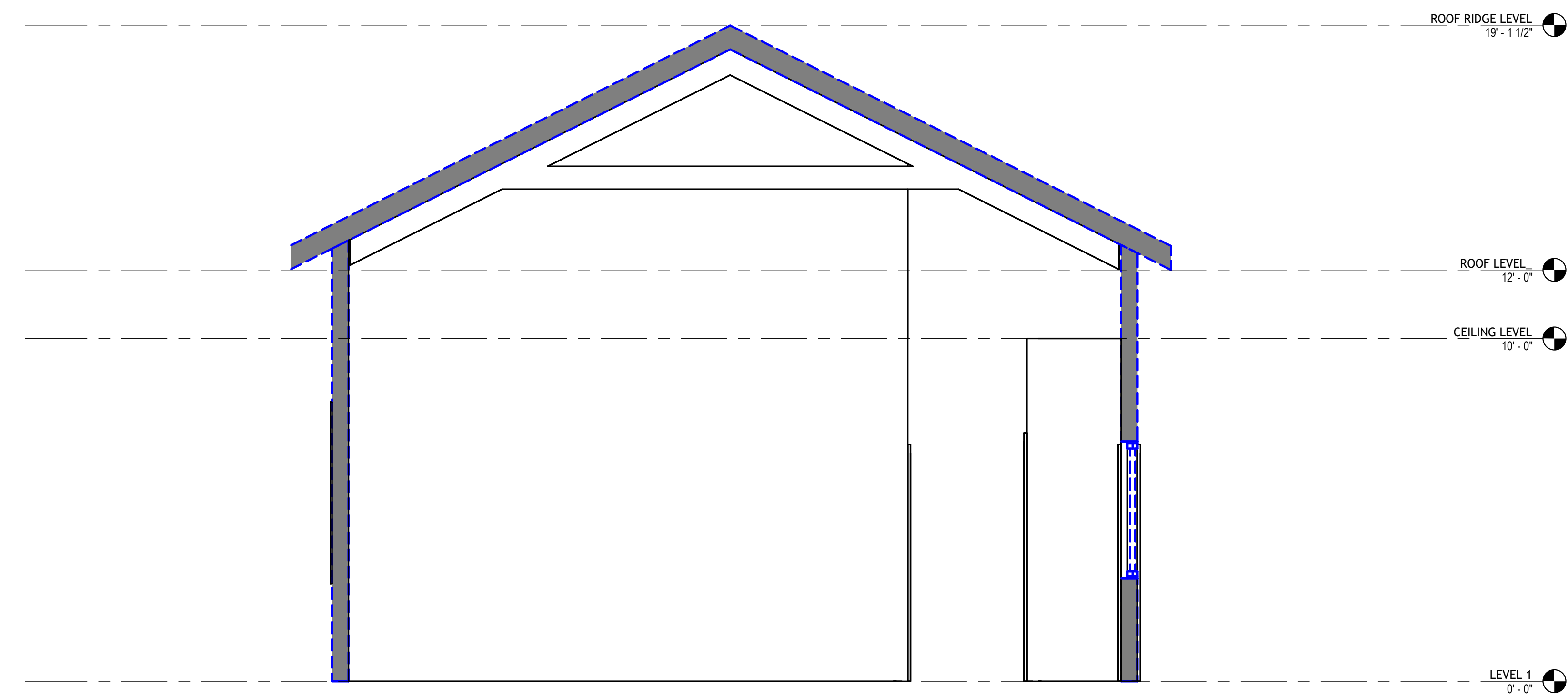
4 | Section 4 3/8" = 1'-0"
