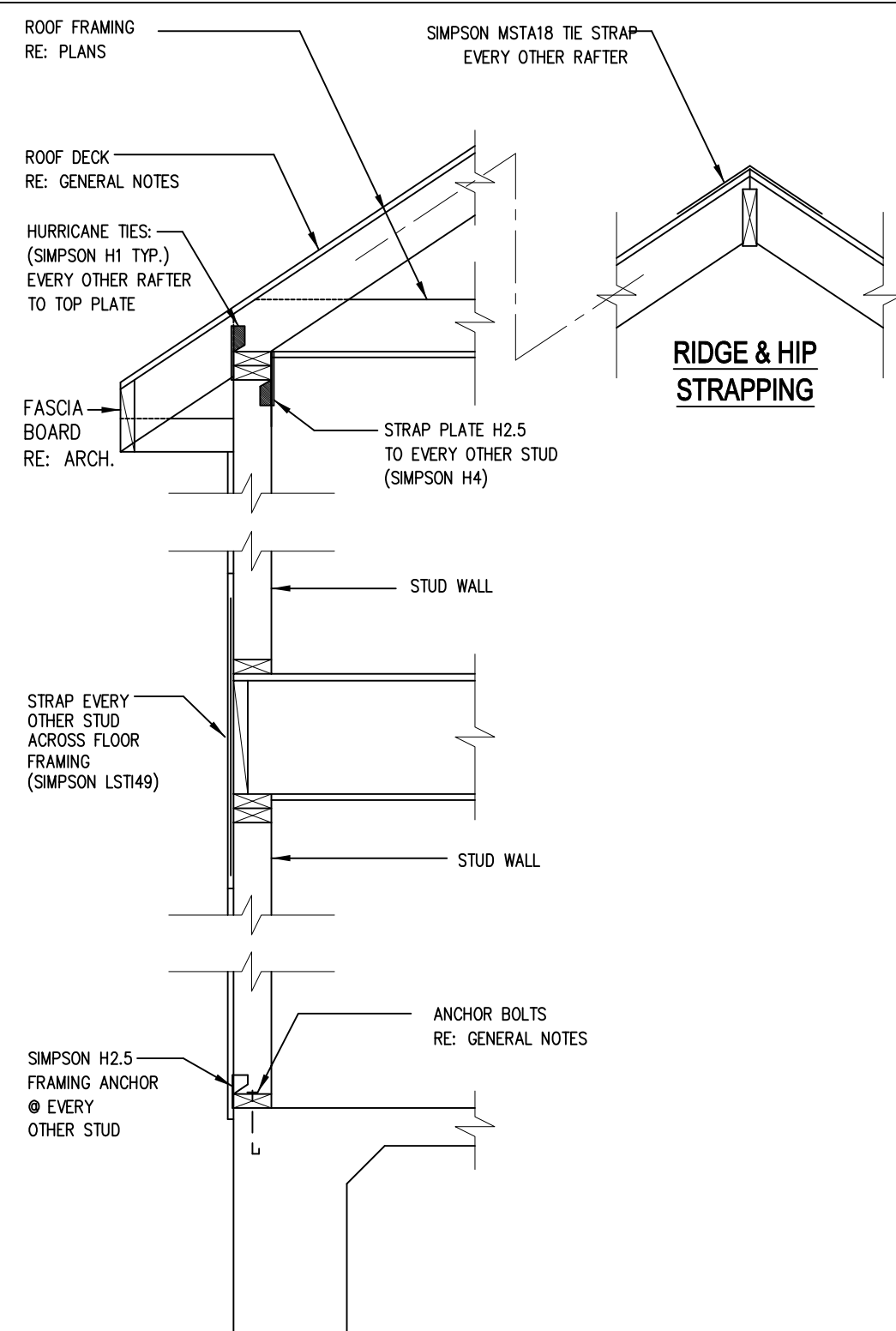
TYPICAL WIND STRAPPING DETAILS (METAL STRAPPING OPTION)
