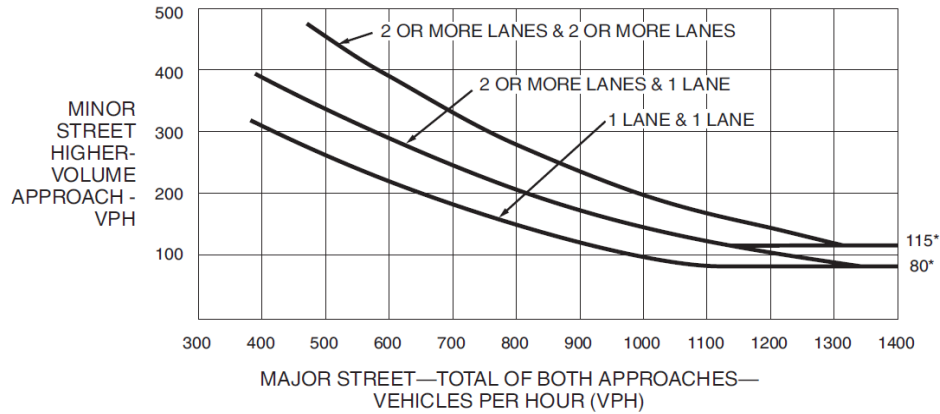
Figure 2 - Warrant 2: Four Hour Vehicular Volumes
