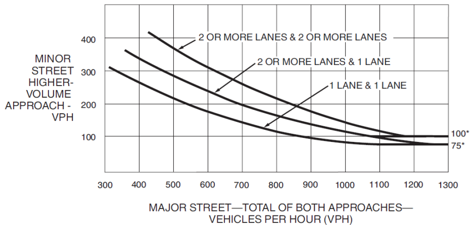
Figure 5 - Warrant 3: Peak Hour Vehicular Volumes (70% Factor) (COMMUNITY LESS THAN 10,000 POPULATION OR ABOVE 40 MPH ON MAJOR STREET)
