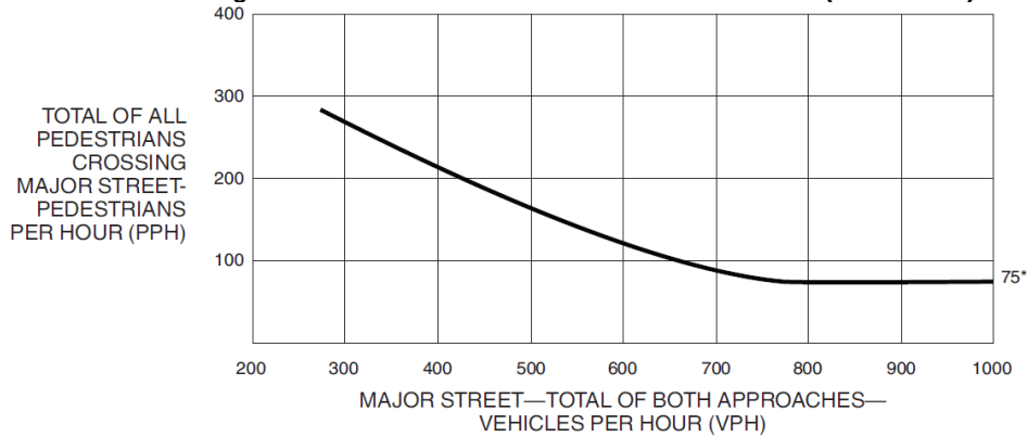
Figure 7 - Warrant 4: Pedestrian Four Hour Volume (70% Factor)
