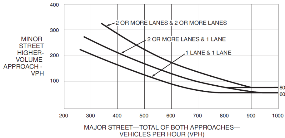
Figure 3 - Warrant 2: Four Hour Vehicular Volumes (70% Factor) (COMMUNITY LESS THAN 10,000 POPULATION OR ABOVE 40 MPH ON MAJOR STREET)
