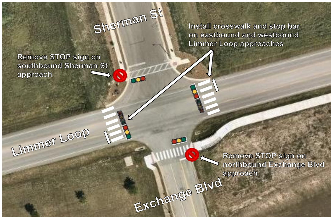
Figure 9: Proposed Intersection Control
