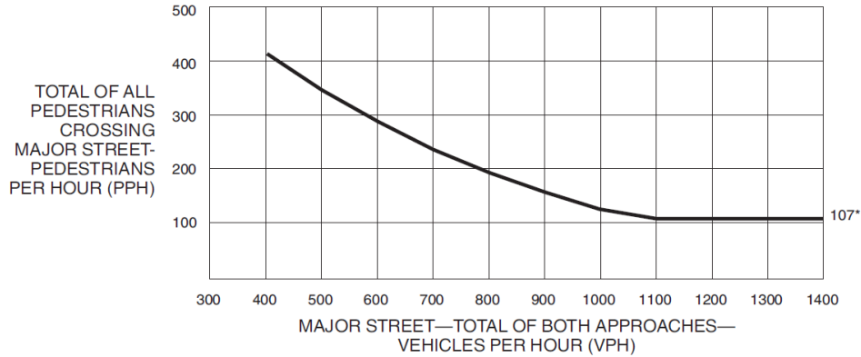
Figure 6 - Warrant 4: Pedestrian Four Hour Volume
