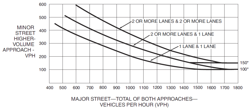
Figure 4 - Warrant 3: Peak Hour Vehicular Volumes
